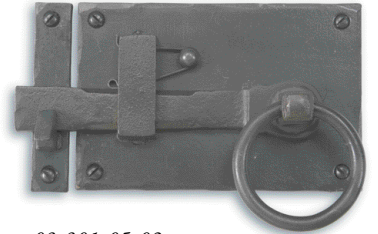
03-301-05-02 Cott Latch With Available with Ring Pulls, Round, Oval or Octagonal Knobs. (Right hand shown). 150mm x 100mm.
