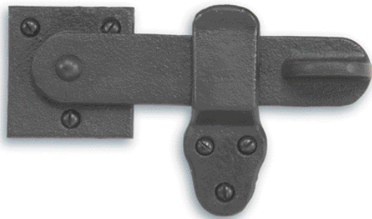
03-400-05 Dartington Door Latch (Operable from one side only) 145mm x 85mm overall.
