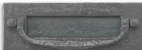
03-500-05 Lincoln Postal Door Knocker 300mm x 105mm overall. Opening 200mm x 44mm.
